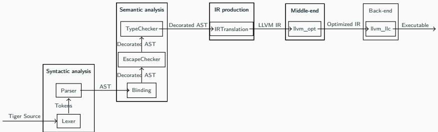
Figure 4: Tiger compiler
